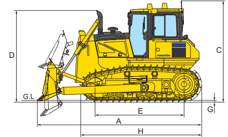
Shown with D65EXi-18 SIGMADOZER® single grouser shoe.
